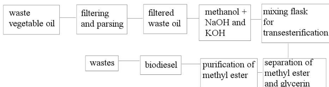
Figure 2. Obtaining biodiesel from waste oils
