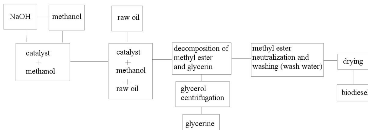
Figure 1. General biodiesel production scheme
