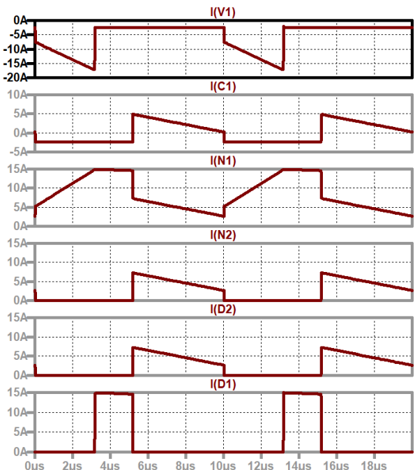
Fig. 7. Steady state (up to down):: current through the source (this current is negative because LTSpice counts current and voltage across a component always in the same direction), current through the capacitor, current through winding N1, current through winding N2, current through the diode D2, current through the diode D1.
